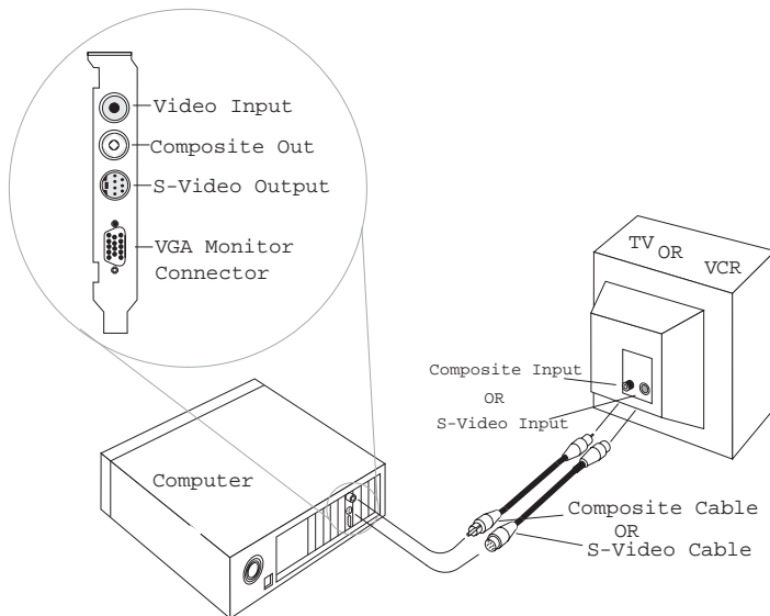
Figure 1. Connecting your ATI graphics card to a TV or VCR
